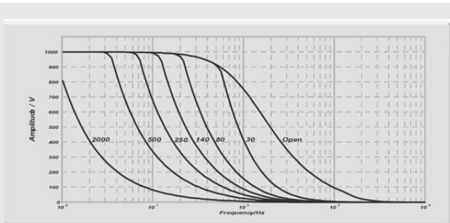
E-463, frequency response with various PZT loads. Values shown are capacitance in nF, measured in actual PZT.
